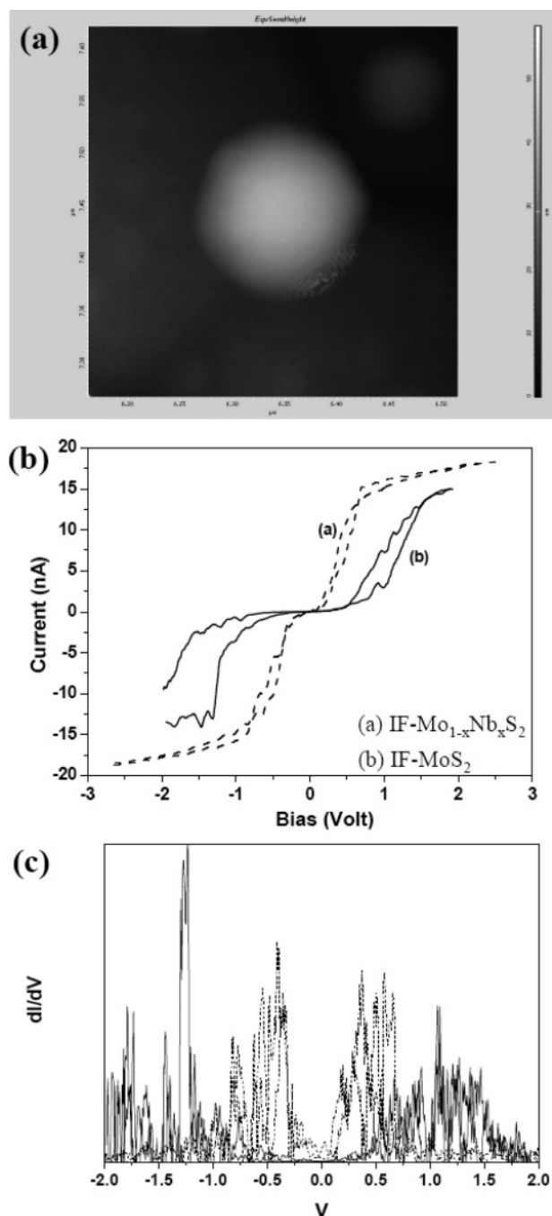
Figure 10. AFM measurements carried out on an IF- Mo_{1-x}Nb_xS_2 nanoparticle (a) AFM image, (b) I/V curves carried out on the nanoparticle (dashed lines), (c) corresponding dI/dV vs V plots. In both (b) and (c), the corresponding plots of the IF- MoS_2 nanoparticle are shown for comparison (solid lines).
