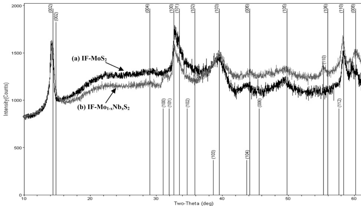
Figure 2. XRD pattern of (a) IF-MoS 2 and (b) nanoparticles prepared at T_1 = 850 °C and T_2 = 900 °C (series 2). Standard diffraction patterns of 2H-MoS 2 (long lines) and 2H-NbS 2 (short lines) are also shown for comparison.
