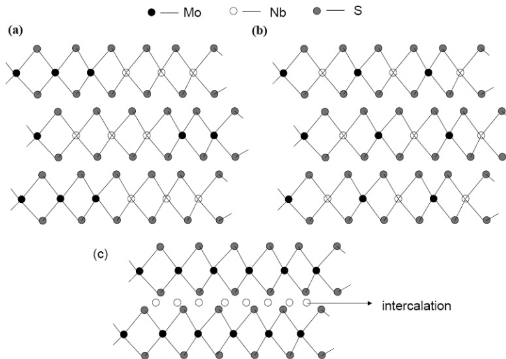
Scheme 1. Substitutional Pattern of the Nb Atoms within the IF- Mo_{1-x}Nb_xS_2 Lattice
