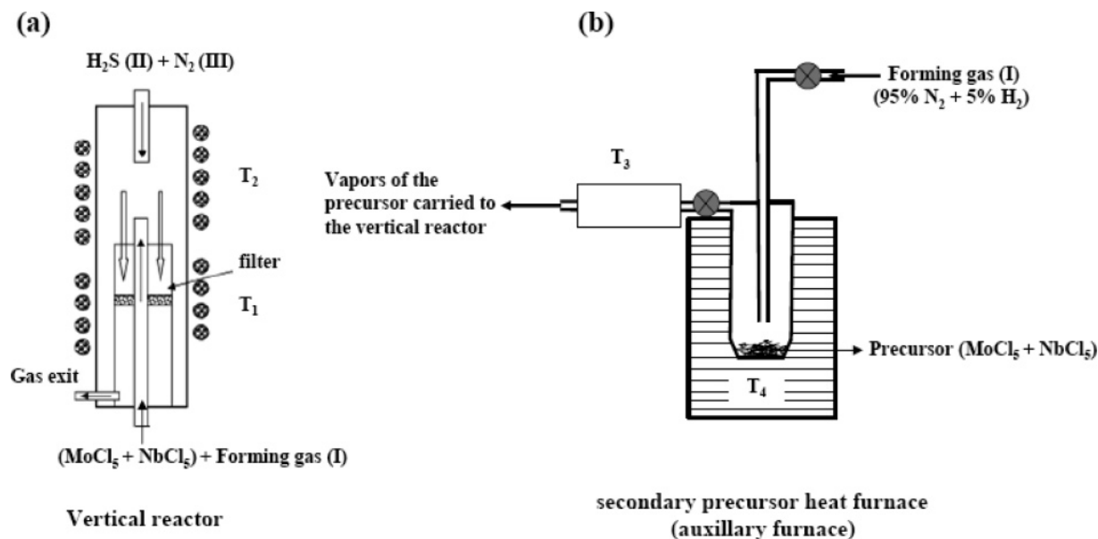
Figure 1. Two-stage furnace setup employed for the synthesis of the IF-Mo 1-x Nb x S 2 nanoparticles. (a) Vertical reactor and (b) the secondary precursor heat furnace (auxiliary furnace).
