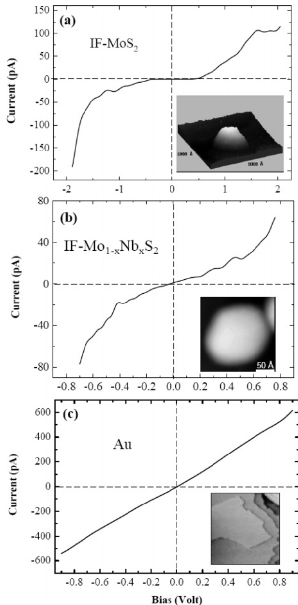
Figure 11. I/V curves at room temperature measured on (a) an IF- MoS_2 nanoparticle ( \sim 40 nm diameter), (b) an IF- Mo_{1-x}Nb_xS_2 nanoparticle ( \sim 30 nm diameter), and (c) the gold substrate. The insets show the corresponding topographic images. The image in (c) is 1 \times 1 mm^2 in size, revealing atomic steps on the Au(111) surface.
