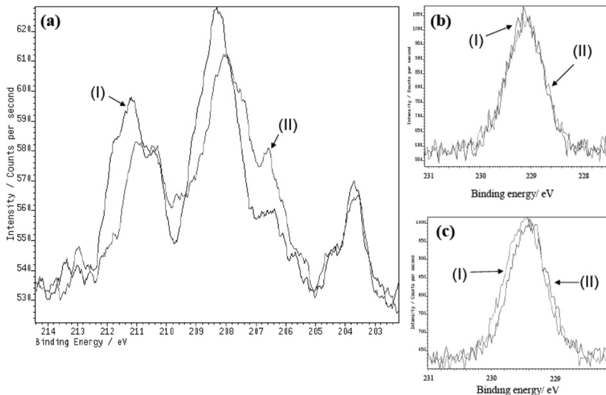
Figure 9. (a) Electrically induced line shifts of (a) Nb(3d), (b) Mo ( 3d_{5/2} ) in IF-Mo _{1-x} Nb _x S _2 nanoparticles, and (c) Mo ( 3d_{5/2} ) in IF-MoS _2 nanoparticles. In all panels, curve (I) corresponds to “eFG off” conditions and curve (II) refers to “eFG on”. Note that (panel a) the oxidized Nb exhibits a large shift while the reduced Nb signal is practically not shifted at all. Comparison of panels (b) and (c) demonstrates the effect of Nb substitution on the Mo line shift, indicating improved conductance in the IF-Mo _{1-x} Nb _x S _2 nanoparticles.
